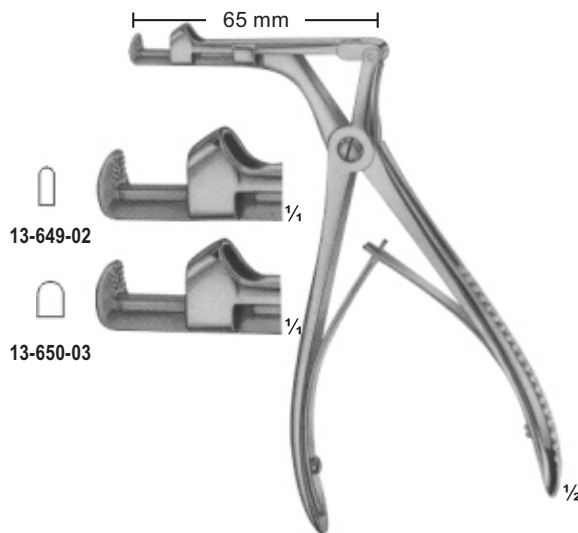
CITELLI 13-649-02 - 13-650-03 13-649-02 2 mm 13-650-03 3.5 mm
