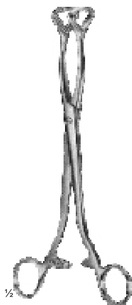
LUER 17-128-22 - 17-129-24 17-128-22 22 cm 17-129-24 24.5 cm
